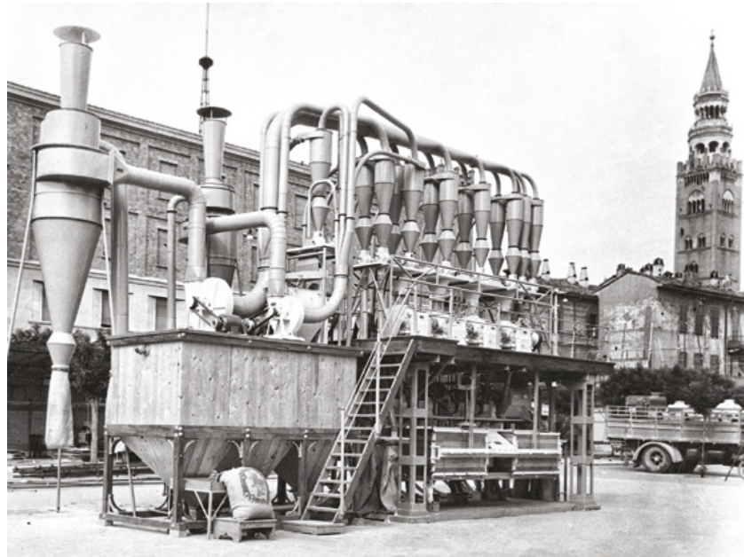
The Superior compact mill in 1948.
